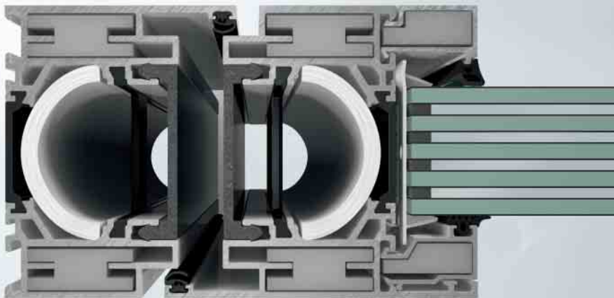
Schüco Tür FireStop ADS 90 FR 90 Schüco FireStop ADS 90 FR 90 door
